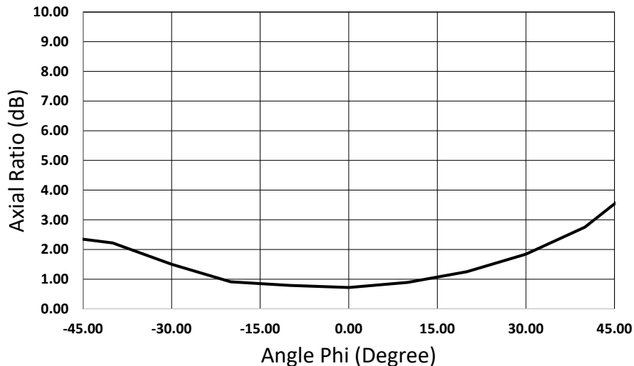
Measured Axial Ratio Versus Angle
