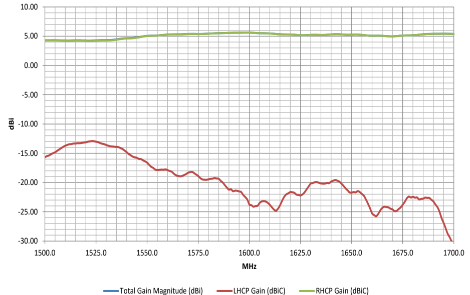
Broadside +Z Axis Gains in dBi
